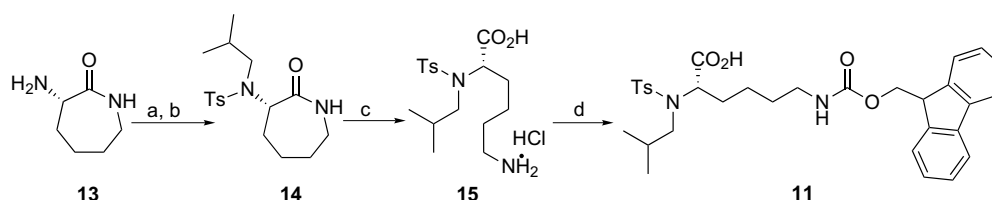
Scheme 1. Reagents and conditions: (a) i -PrCHO, MeOH, NaCNBH 3 , pH 4; (b) TsCl, NEt 3 , CH 2 Cl 2 , 88% (two steps); (c) 6 M HCl, reflux; (d) FmocOSuc, K 2 CO 3 (1 M), THF 82% (two steps).
